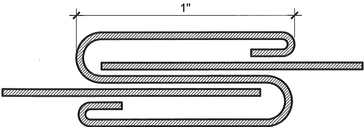
HEMMED "S" SLIP
