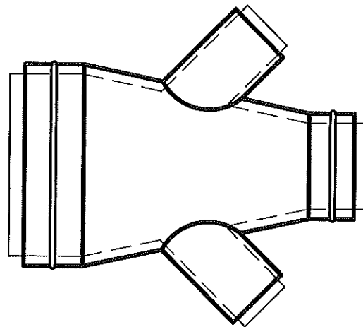
REDUCER WITH TAP @ 45°
