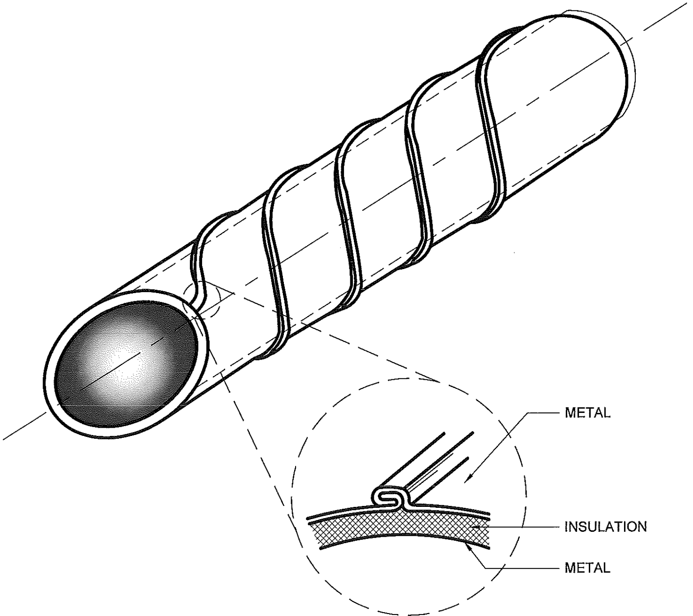
SPIRAL SEAM
